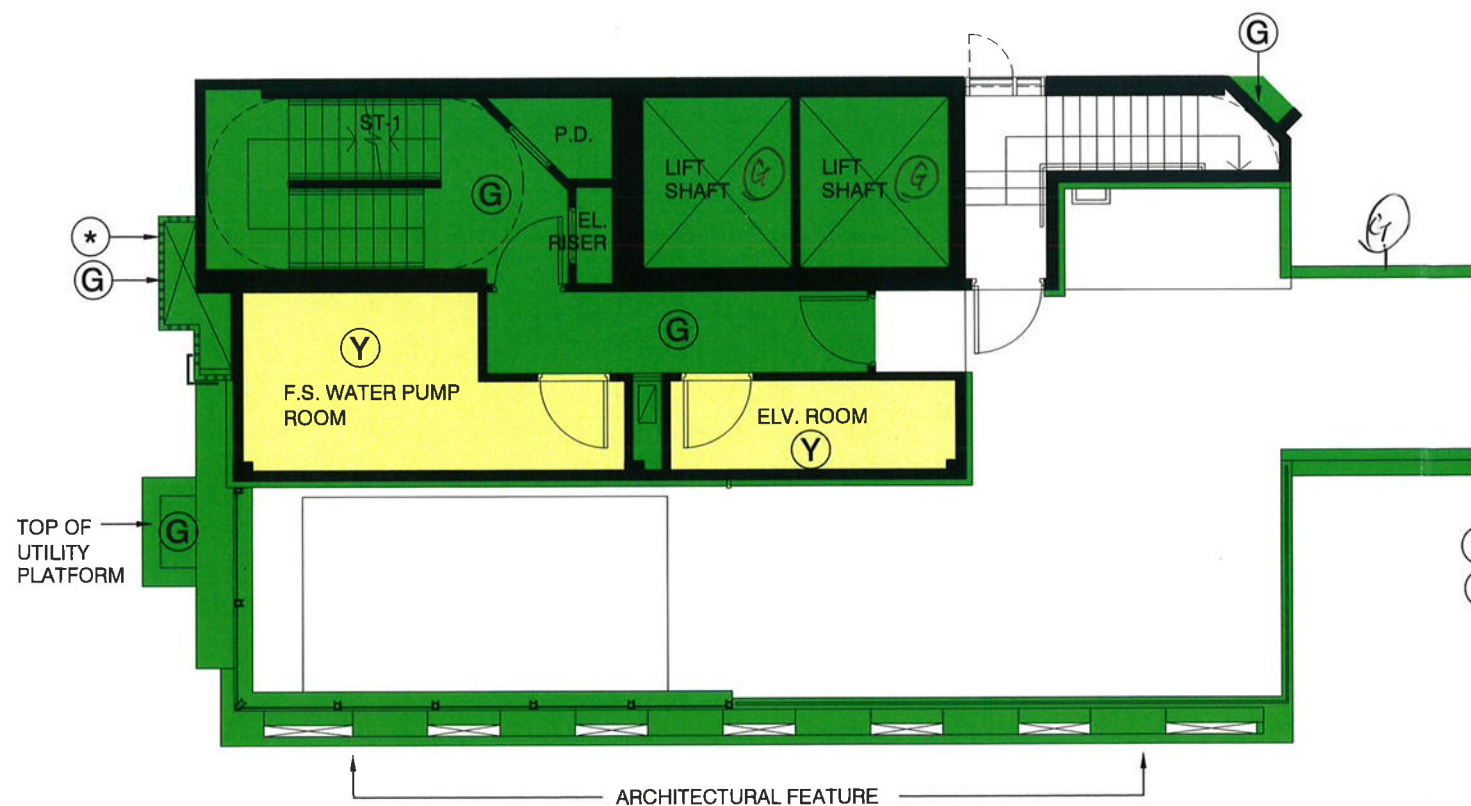
ROOF PLAN
